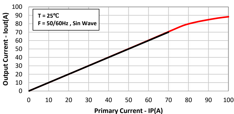
DWCS3300 I AC V.S. I P at V DD 5V
