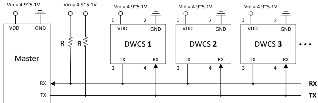
App. 3 Modbus Connection
