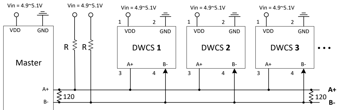
App. 5 RS485 Connection
